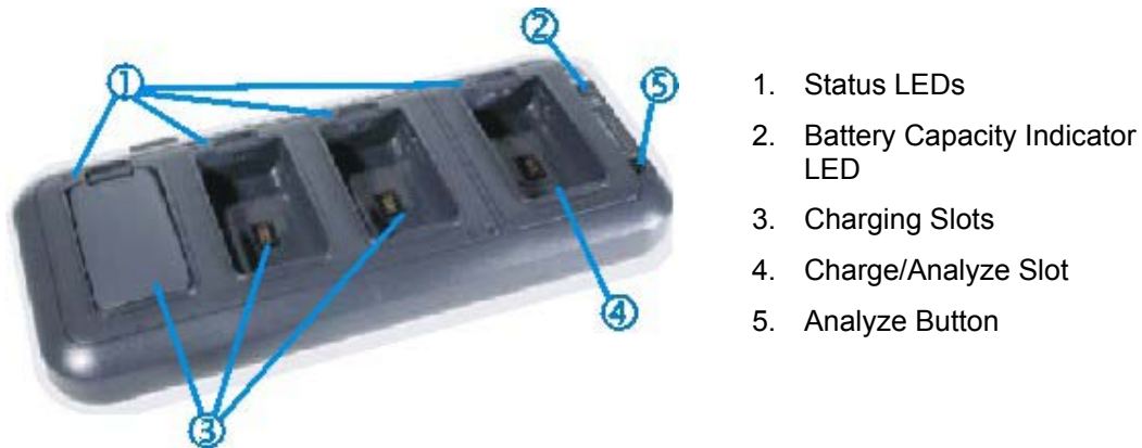
Figure 20 Multicharger / Analyzer
