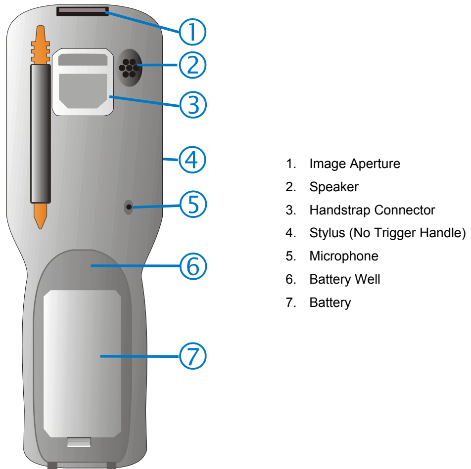
Figure 2 Back of MX6
